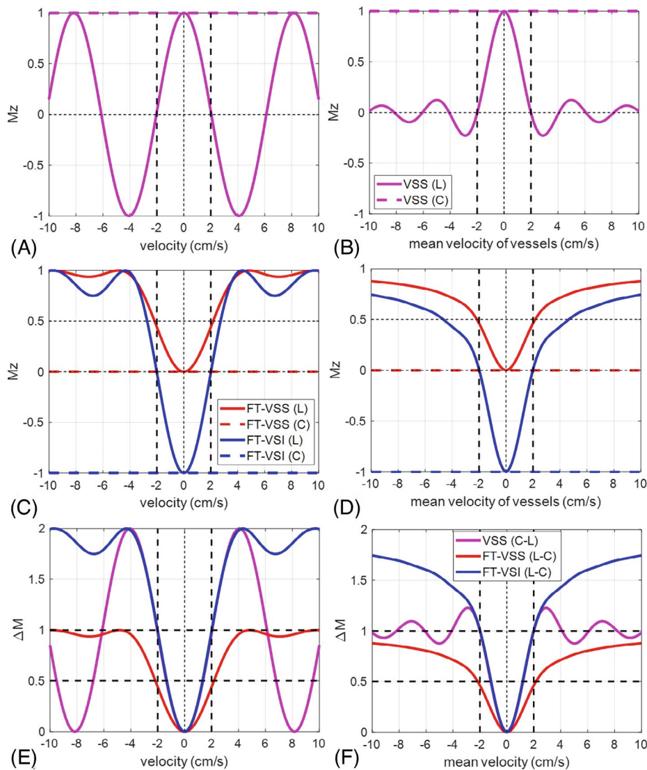
FIGURE 6 Simulated M_z -velocity responses of (A) velocity selective saturation (VSS) (magenta), (C) Fourier transform (FT)-VSS (red) and FT-velocity selective inversion (VSI) (blue), and (B, D) the corresponding results after the laminar flow integration (note that the x-axis is the mean velocity). The horizontal dashed lines are their magnetization responses under the control, respectively. Their arterial spin labeling (ASL) subtractions ( \Delta M ) between label (L) and control (C) are displayed before (E) and after (F) laminar flow integration as well. V_{\text{cut}} is defined as the first crossing of \Delta M = 1 , as indicated by the vertical black dotted lines at 2.0 cm/s (E,F). For VSS, the V_{\text{cut}} is chosen under the assumption of laminar flow (F). This point is the first 0-crossing of the velocity response under the label condition (B). For FT-VSI, V_{\text{cut}} can be defined without using laminar flow model (E). This is also the 0-crossing or half-width-half-maximum point of FT-VSI's velocity response under the label condition (C)
